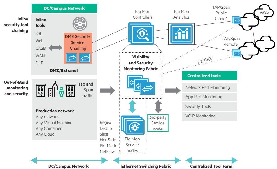
Figure 1. Big Monitoring Fabric—Architecture
